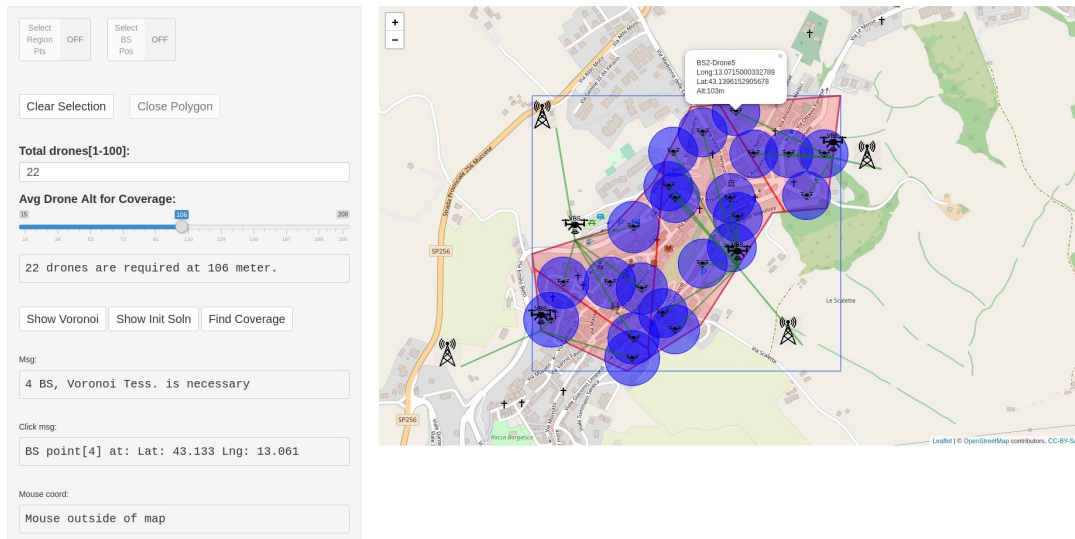
Figure 2.1.4: The GUI of the prototype simulator.
