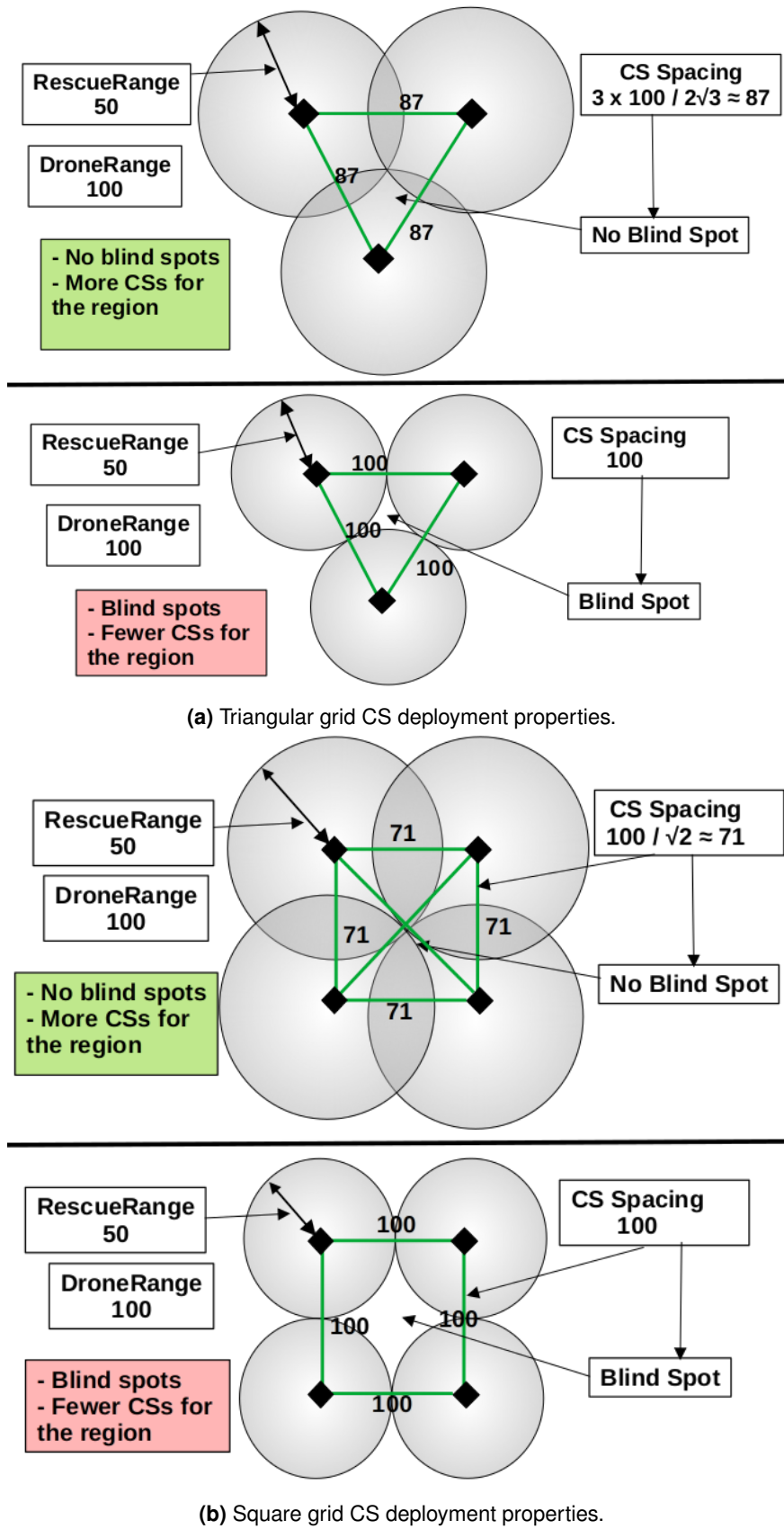
Figure 3.1.5: CS grid deployment properties.
