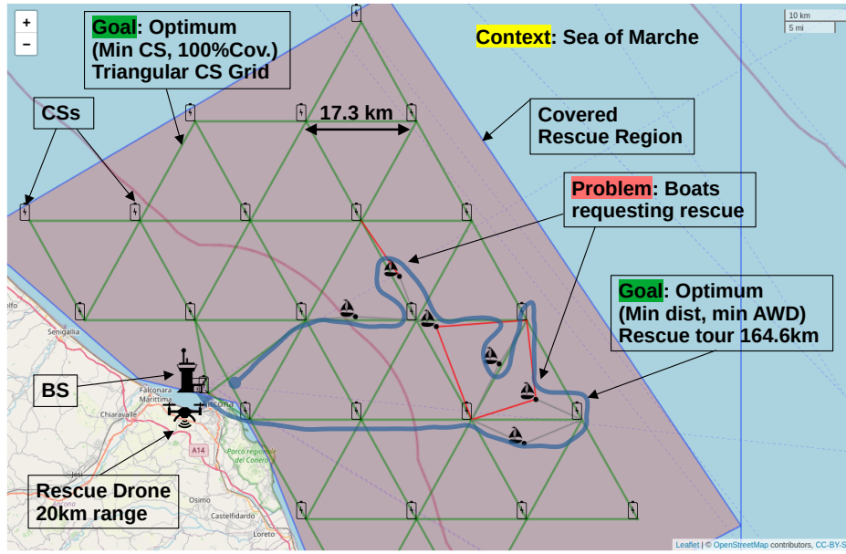
Figure 3.1.2: Boat rescue operation with drones.
