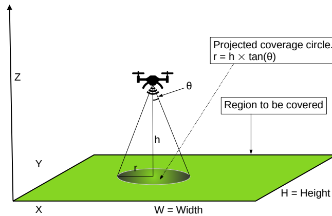
Figure 1.0.5: Drone altitude - projected circle on the ground relationship.
