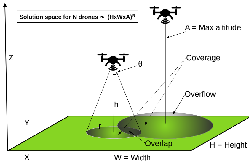
Figure 2.1.1: Individual drone parameters for coverage missions.
