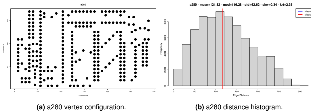
Figure 3.2.16: a280 dataset.
