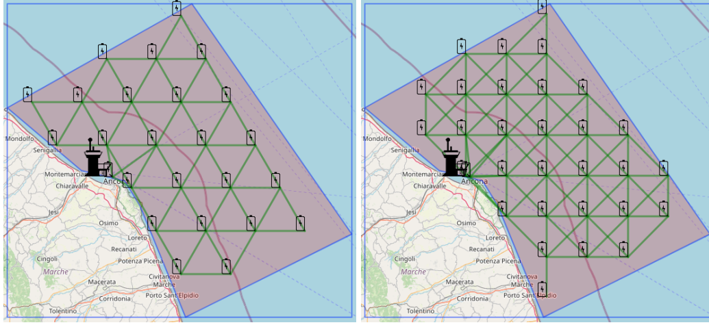
(a) Actual triangular CS Grid deployment (24 CS). AVG SP length from BS = 2.06 units. (b) Actual square CS Grid deployment (30 CS). AVG SP length from BS = 2.07 units.
