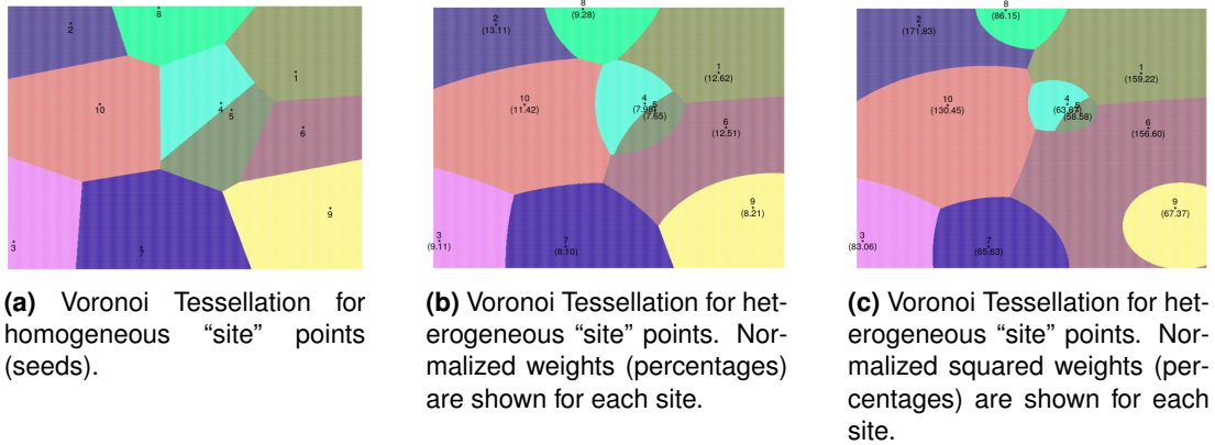
Figure 2.1.3: Voronoi Tessellation alternatives for different coverage schemes.
