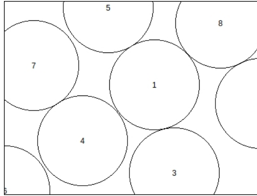
Figure 2.4.1: Initial solution for 8 drones (hexagonal circle-packing algorithm). Cov: 75.61%. TDist: 2457.35 m. Time: < 1 sec.
